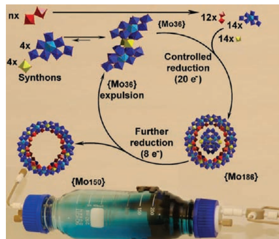
Figure 2. Scheme showing the assembly of a MB nanoring, complete with {Mo 36 } template under continuous flow conditions. Color scheme: {Mo 1 }, yellow; {Mo 2 }, red; {Mo 8 }, blue (central MoO 7 pentagonal bipyramid, light blue). Background shows the flow reactor setup used in our studies.
