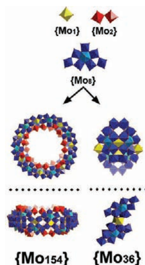
Figure 1. Scheme showing the assembly of the parent MB nanoring {Mo 154 } (left), and the {Mo 36 } unit (right) from transferrable building blocks. Color scheme: {Mo 1 }, yellow; {Mo 2 }, red; {Mo 8 }, blue (central MoO 7 pentagonal bipyramid, light blue).
